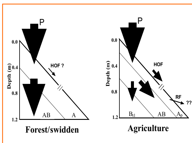
Figure 20: Schematic representation of precipitation (P) partition into deep percolation, lateral flow, Horton flow (HOF) and return flow (RF). ? refers to the insignificance of the flow component (Ziegler 2007).
