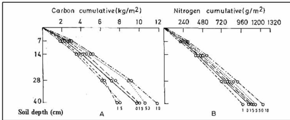
Figure 2 Changes in cumulative quantity of carbon (A) and nitrogen (B) within a soil column of 40-cm depth under 0-, 1-, 5-, 10-, 15- and 50-year old jhum fallows (after Ramakrishnan & Toky 1981)
